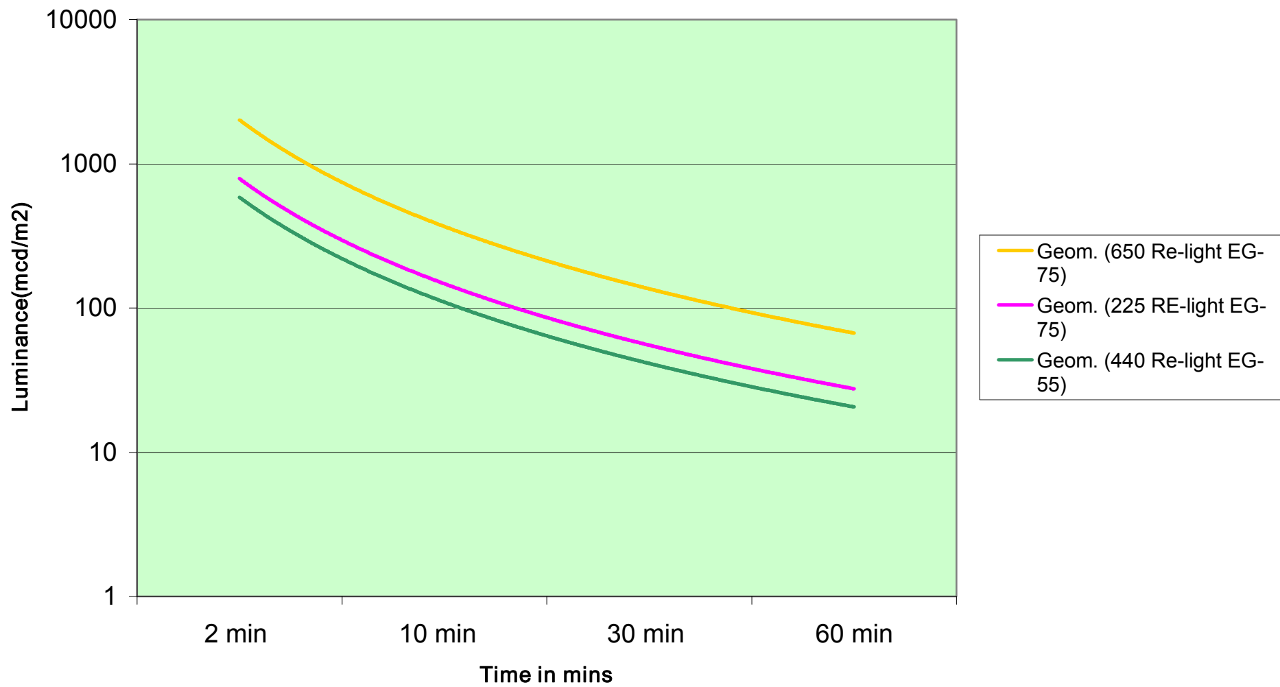
The various RE-light products tested after ISO 67510 - 1992 by SP, Sweden
